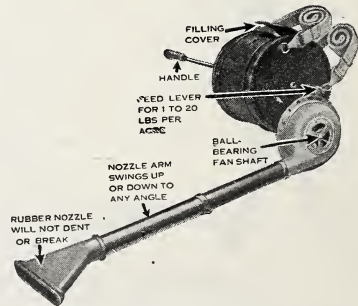
SMITH SAVAGE DUSTER
